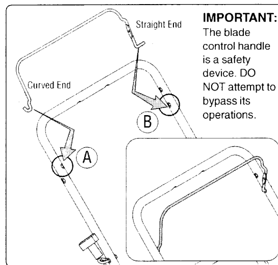
Figure 5: Attaching the blade control handle (optional)
