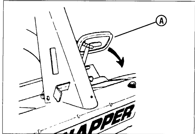
Figure 5: Engaging the clutch/brake pedal
