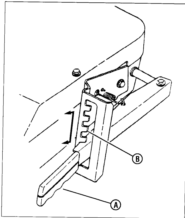
Figure 18: Cutting height adjustment
