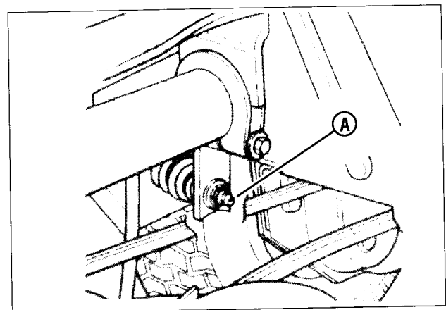
Figure 26: Shift lever grease fitting
