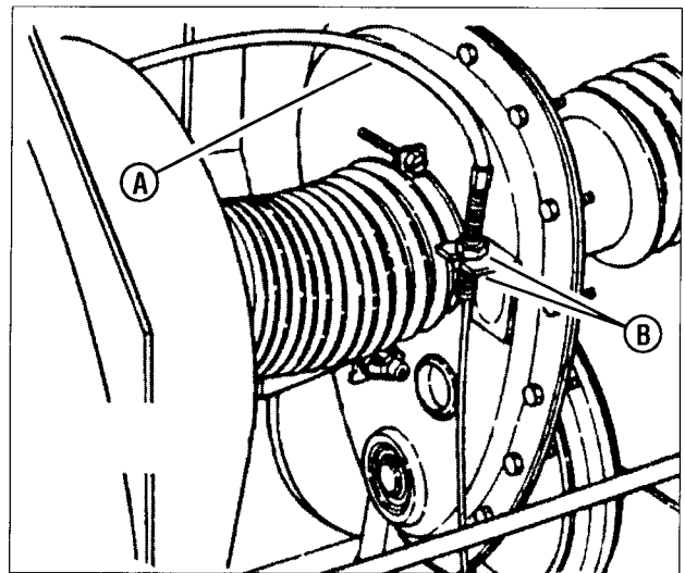
Figure 41: Brake cable adjusting nuts
